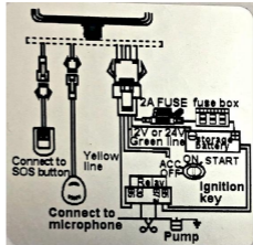
Optional MIC and SOS wiring diagram
